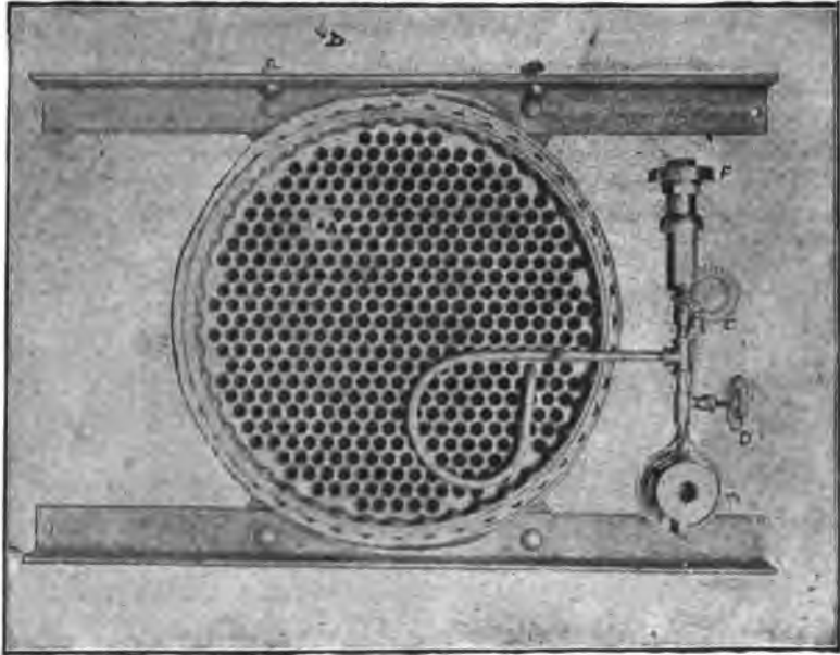
FIG. 150.—Bottom View of the "Reading" Carriage Boiler, showing the arrangement of the flues in the crown sheet; also, method of riveting on the head, non-conducting boiler lagging, and attachment of boiler to two angle iron supports running in the width of the carriage. The liquid gasoline is fed from the storage tank through a tube passing to the top of the boiler, thence down through one of the flue tubes, and, in the loop, here shown, over the burner flame, into the regulator and distributor. F is the automatic fuel regulator; E, the preliminary vaporizing coil; C and D, valves controlling the feed; A, the fusible plug. The operation of the fuel feed will be explained in the chapter on burners.
